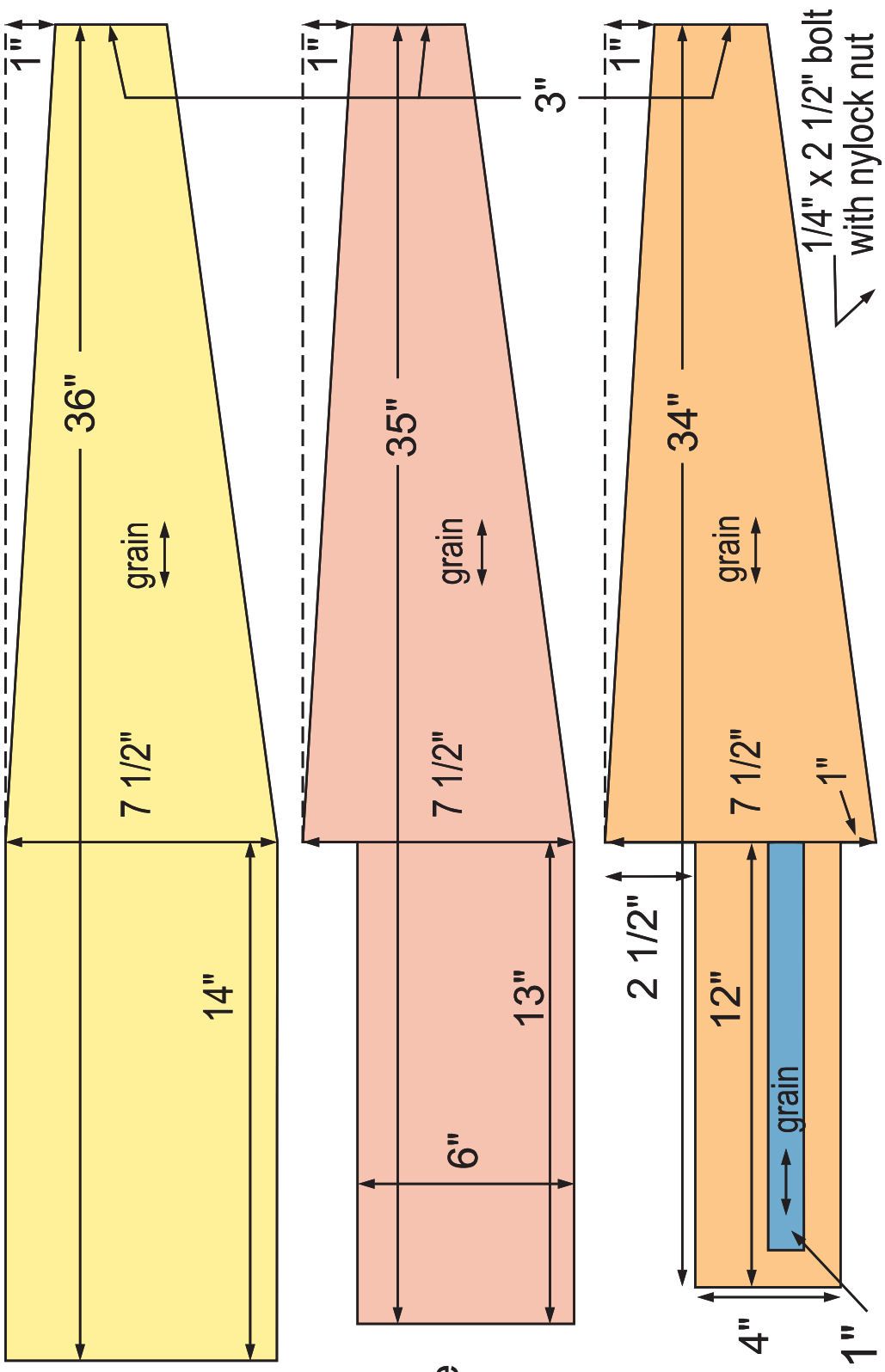
NACA 0012 8" rudder made from layers of 1/8" plywood
